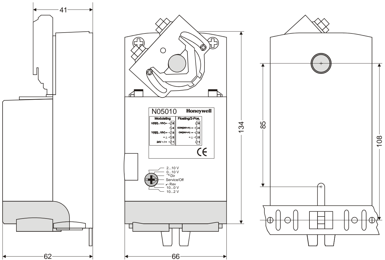
Fig. 15. Dimensions (in mm)
