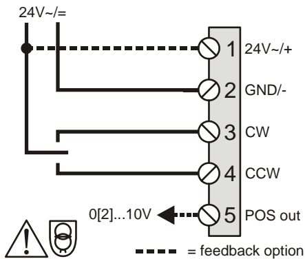
Fig. 12. N05010/N10010 (floating mode)
