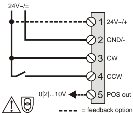
Fig. 13. N05010/N10010 (2-position mode)
