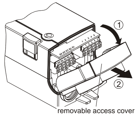
Fig. 10. Access cover
